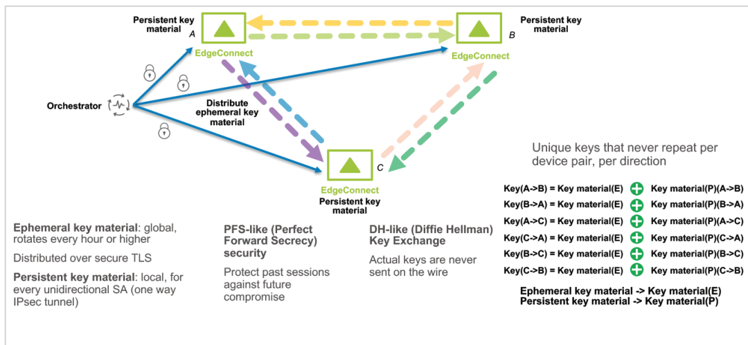
Figure 3: Silver Peak IPsec Key Management
