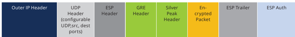
Figure 10: IPsec UDP (ESP) packet with Silver Peak encapsulation
